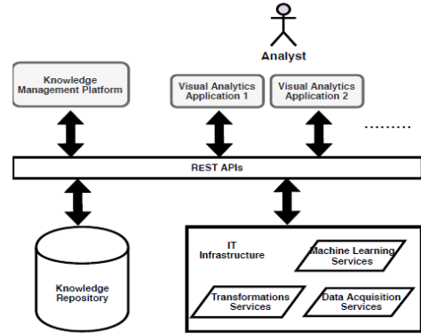
Fig. 6. Proposed Architecture that integrates a knowledge repository and current IT infrastructure as services via REST APIs [22]
