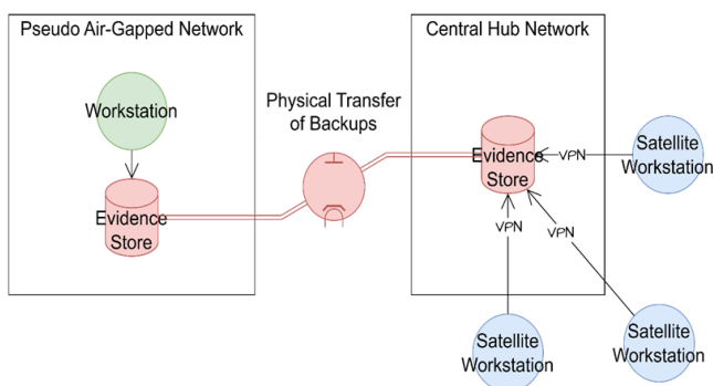
Fig. 5. System Architecture
