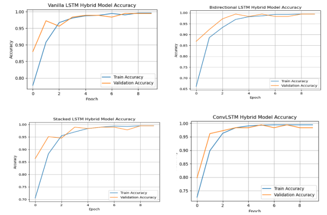
Fig. 5. Training Accuracy Plots for each LSTM Model
